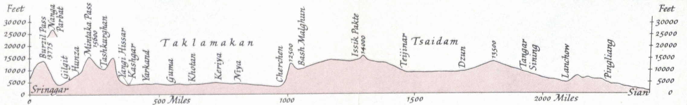
Section along line of Route
